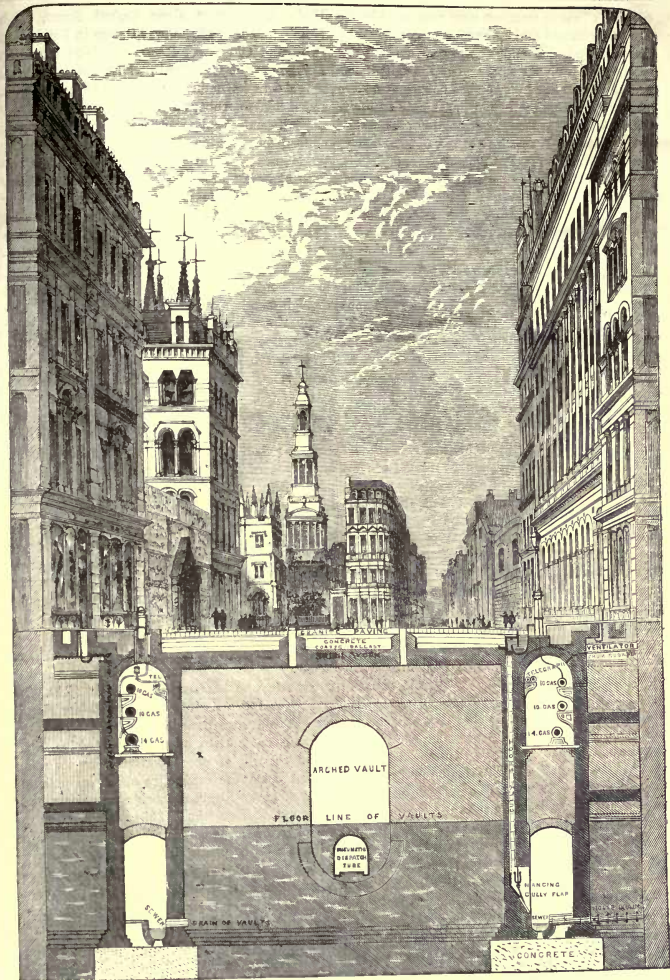
SECTION OF THE HOLBORN VIADUCT, SHOWING THE SUBWAYS.
